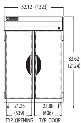
VSR-2 FRONT VIEW
