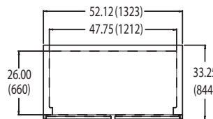
VSR-2 TOP VIEW
