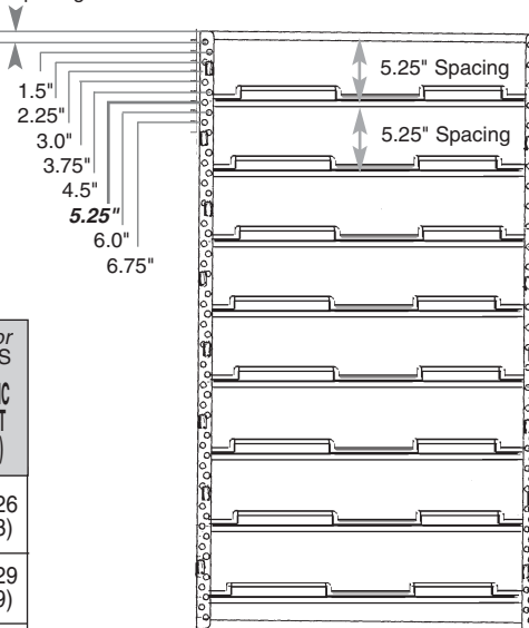
Side View of ETC-1520-16
