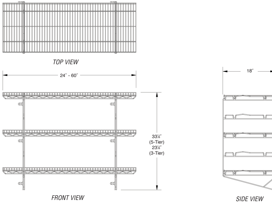
5-tier bracket kit shown with 3 shelves - S3-5B-SSW1848C
