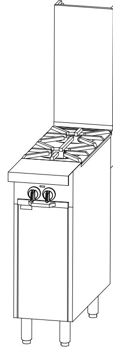
Model P12C-B with optional 24" flue riser
