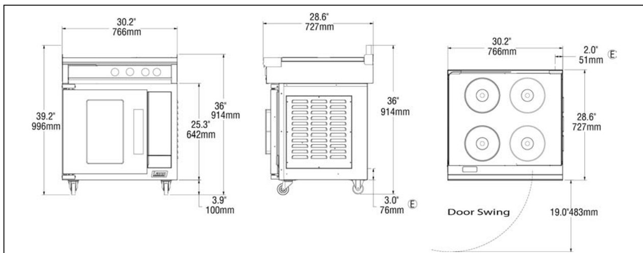
[Front View/Elevation]
