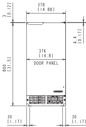
FRONT DIMENSIONS (ADA compliant unit)
