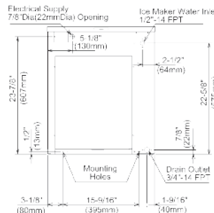
AIR-COOLED UNIT
