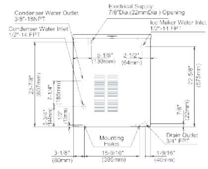
WATER-COOLED UNIT
