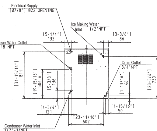
WATER-COOLED UNIT
