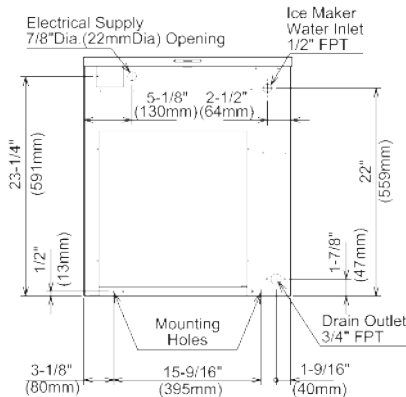
AIR-COOLED UNIT
