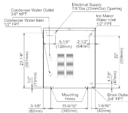
WATER-COOLED UNIT
