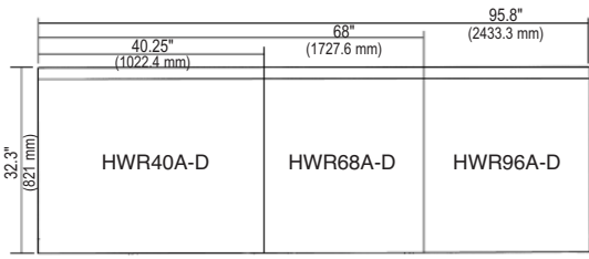
PLAN VIEW (ALL UNITS)
