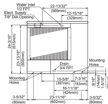
AIR-COOLED UNIT
