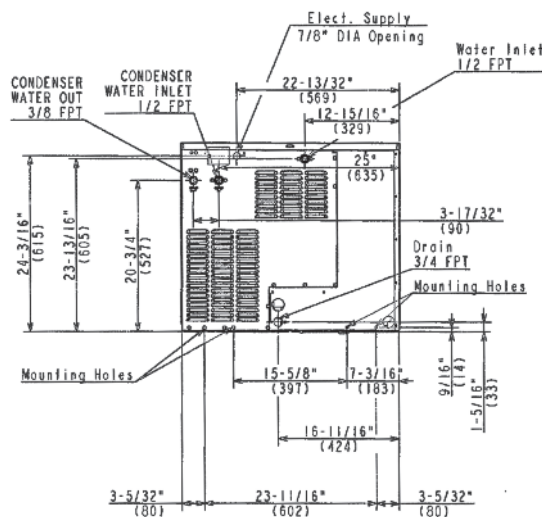
WATER-COOLED UNIT
