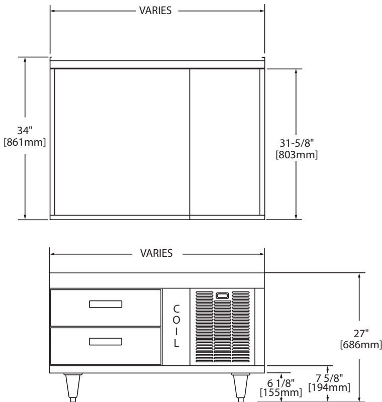
27" DRAWER
