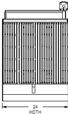
Heavy Duty Cookline Lava Rock Charbroiler Model BPHCRB-2424i
