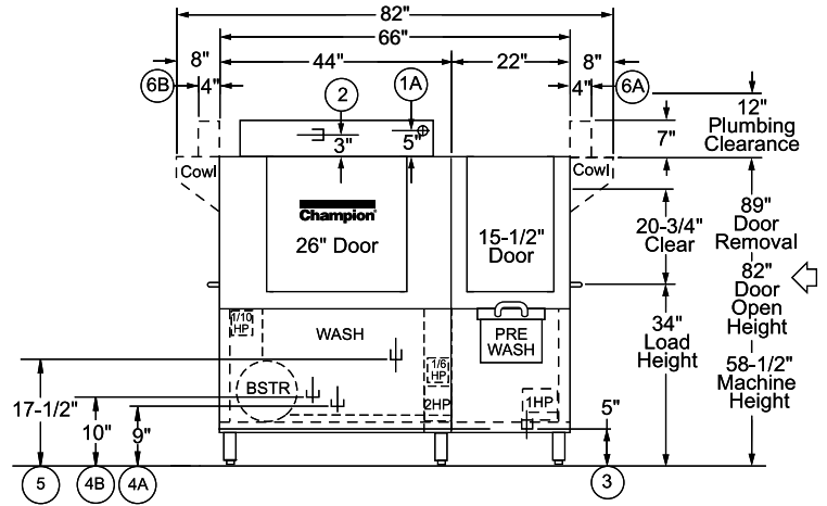
Front View With Booster
