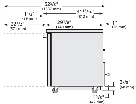
RIGHT VIEW
